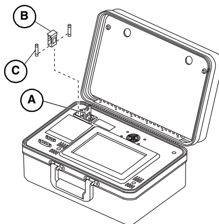
Figure 70 – Fuse Replacement
